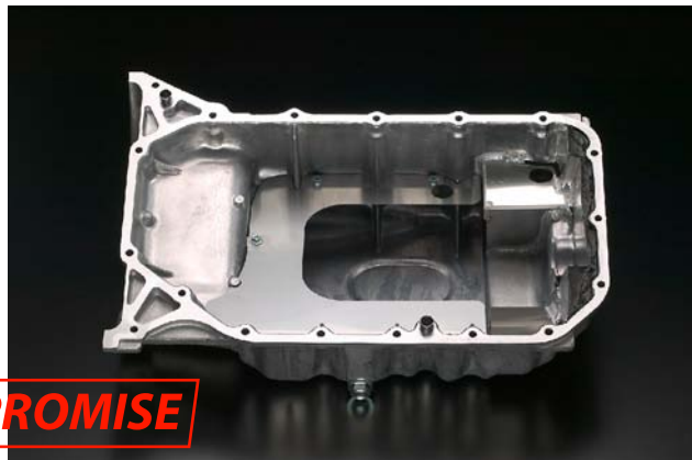
Anti G force oil pan K20A DC5/EP3
