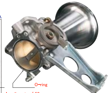
Throttle valve diameter \phi 50mm & also \phi 45mm available.
