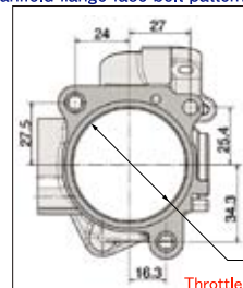
Throttle valve diameter \phi 50mm & also \phi 45mm available.
