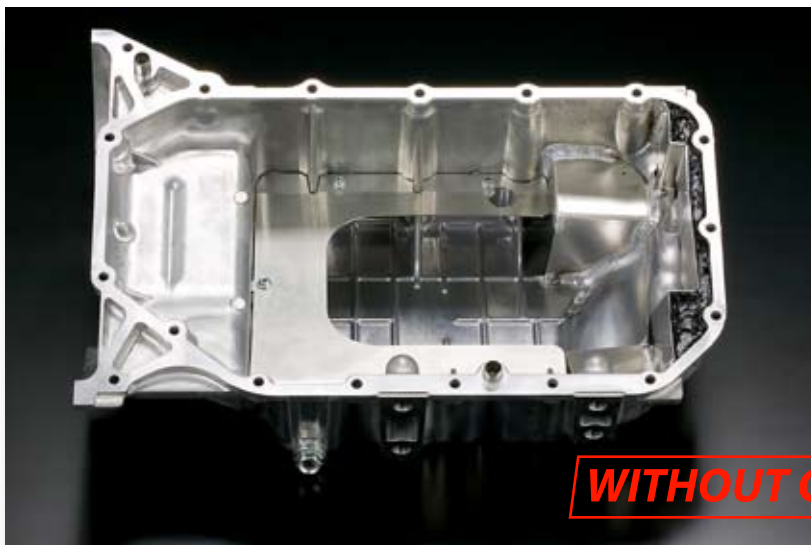
Anti G force oil pan K20A FD2 CIVIC-R
