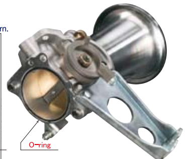
Throttle valve diameter \phi 50mm & \phi 45mm available.
